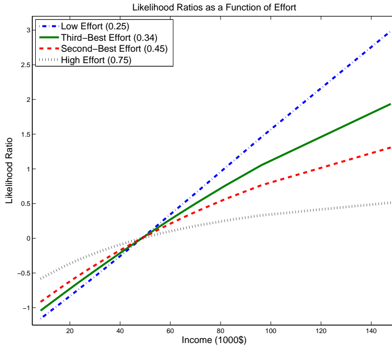
Figure 4: Likelihood ratio function implied by the estimated parameters of the labor income taxation model
